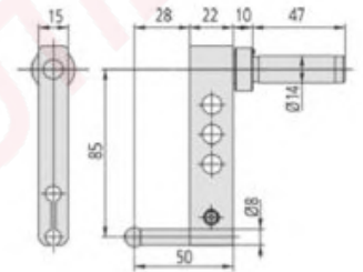
12AAA793 (support long)
