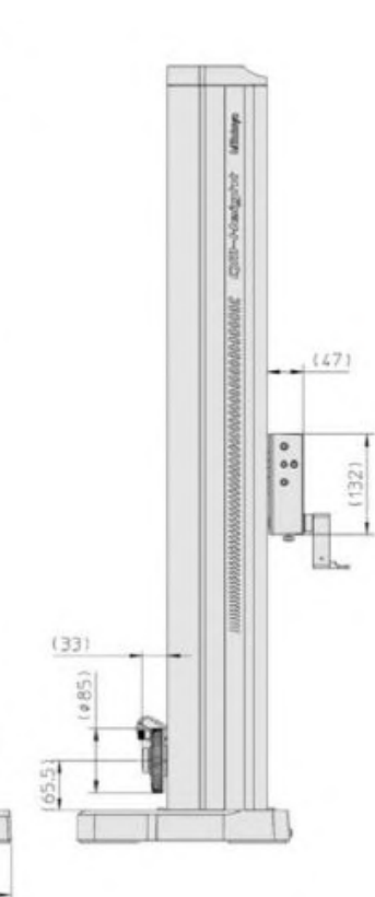
12AAA793 (support long)
